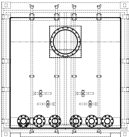
L20 VESSEL END VIEW
